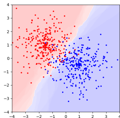
k = 11
